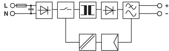
Figure 2 Block diagram
